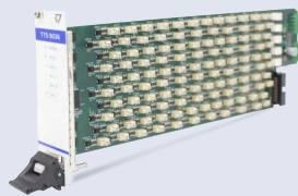
Resistor Board
